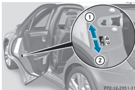
Child-proof lock, rear door (example: Sedan)
