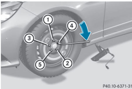
Tightening the wheel nuts (example: vehicle with an emergency spare wheel)
